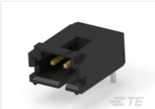
TE Part # 5-104935-3 03 MTE HDR SRRA LATCH
