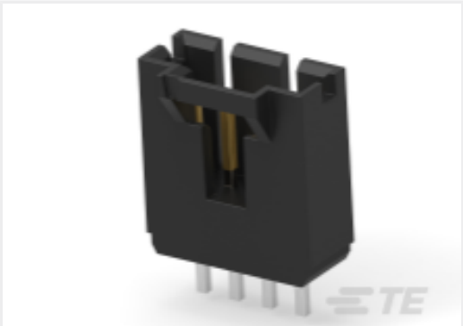
TE Part # 5-103735-3 04 MTE HDR SRST LATCH .100CL
