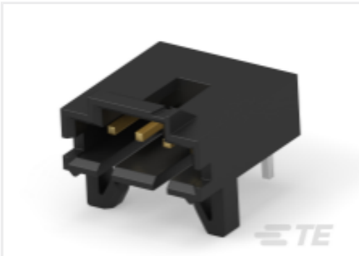
TE Part # 5-103673-3 4 MTE HDR SRRA LATCH W/HLDWN
