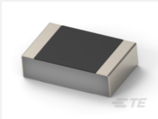
TE Part #7-2176453-7 CPF 0201 35K7 0.1% 25ppm 1K RL
