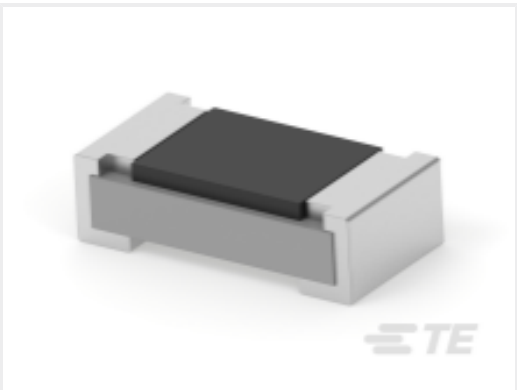
TE Part #1-2176237-0 CPF A 0603 47R 0.1% 25PPM 5K RL
