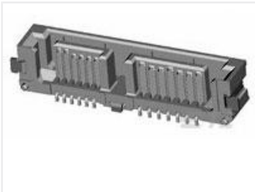
TE Part #1735471-3 Assembly Slimline SATA Plug 7P+6P
