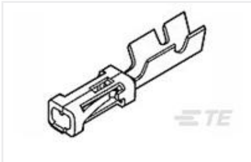
TE Part #167023-1 MOD-4 REC.CONTACT
