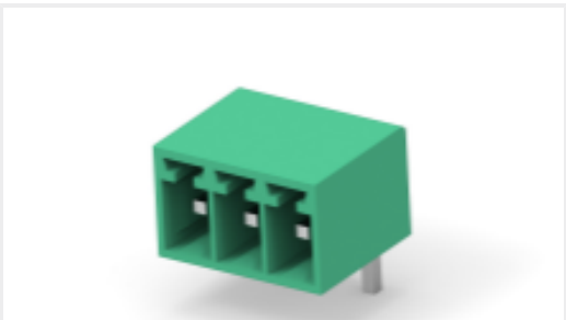
TE Part #2350514-3 3POS TB HDR 90 DEG, PITCH 3.5 & TL 3.5mm
