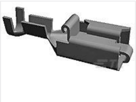
TE Part #927854-8 POSITIVE LOCK REC 1.0-2.5MM2 SILVERPLATE
