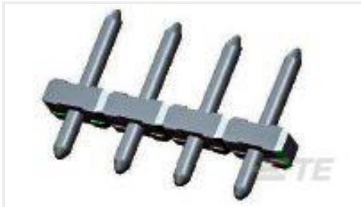
TE Part #1-1546931-0 10P UNSHROUD 5.0 HDR,HIGH TEMP
