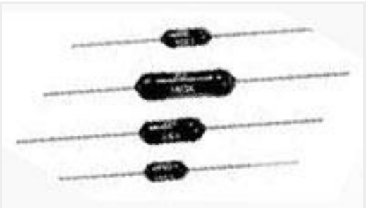
TE Part #3-1879625-4 H8 240R 1% 50PPM
