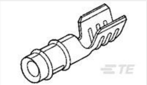
TE Part #640259-1 058 PIN REC IS 18-22 010TP
