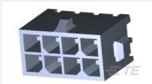
TE Part #3-794630-8 08P MICRO MNL ASSY VRT HDR LF
