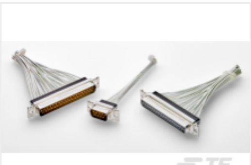
TE Part #2335891-1 AMPLIMITE SZ 1 PLUG 15 POS, ST STL SHEL
