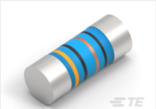
TE Part #7-2176316-0 MELF SMA_A 47K 1% 50PPM 0207 1W
