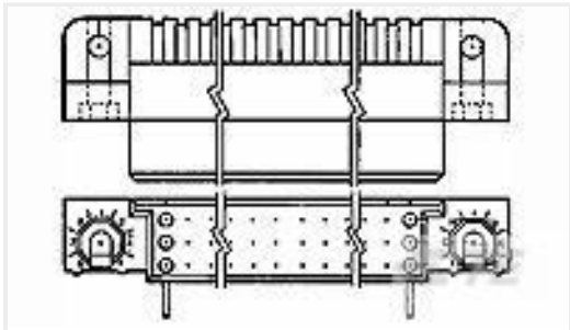
TE Part #533268-8 HDI RECP ASSY 3 ROW 165 POS
