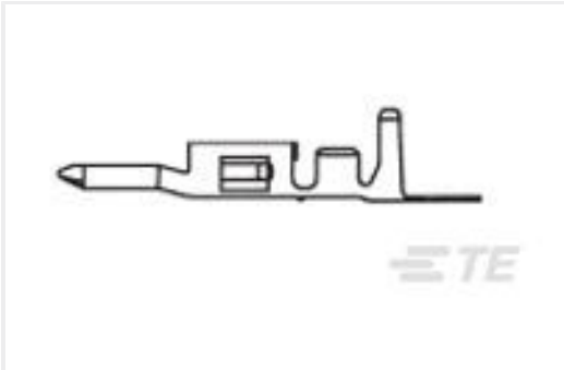
TE Part #1586314-3 VAL-U-LOK PIN PHBZ SN 24-18 LP
