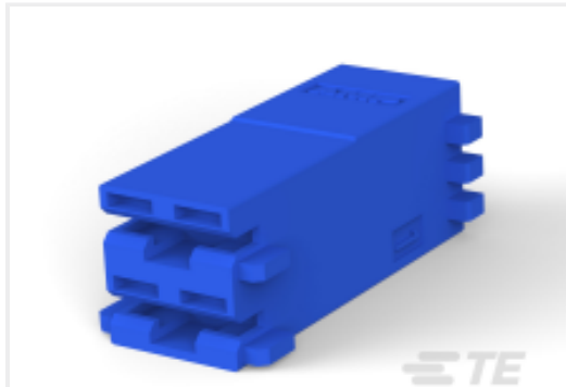
TE Part # 521204-8 RAST 5,HSG,2P,POSILOCK MKIII
