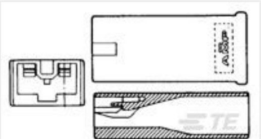
TE Part #41802 250 FASTON FLAG REC 18-12 AWG TPBR
