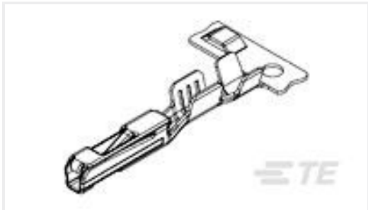
TE Part #1326028-1 0.64MM FEMALE CONTACT,AU,18-20
