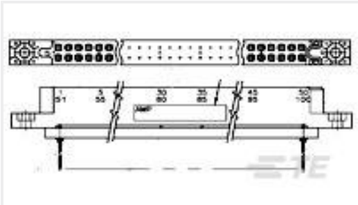
TE Part #534650-9 BOX RECP 110 POS STAG SEALED
