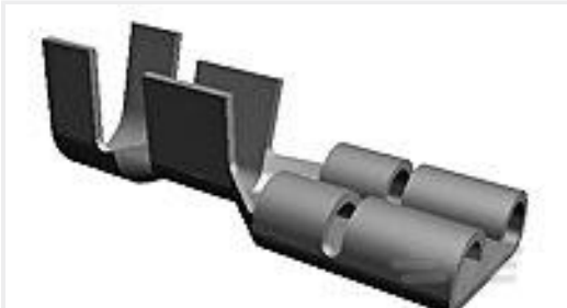
TE Part #62057-1 250 FASTON FLAG REC 12-10 AWG SPBZ
