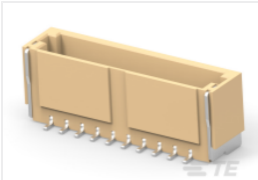
TE Part #1-2473274-0 1.0 WTB SR VT HDR 10 POS
