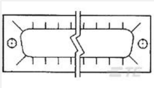
TE Part #745776-4 RFI GASKET,SZ 3,PLTD TIN
