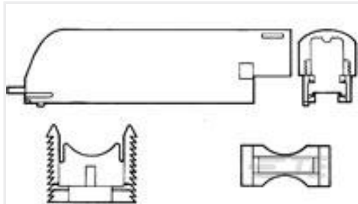
TE Part #552760-1 COVER,90 DEG,SLIDE-ON,"C/PKG"
