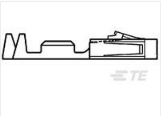
TE Part #104479-8 SHORT POINT CONT PLTD SN
