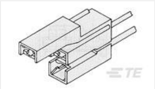
TE Part #360010-1 187 FASTON HSG.,REC.,3 POS, NATRUAL
