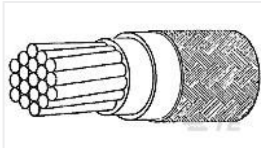
TE Part #262029-001 81044/6-16-9
