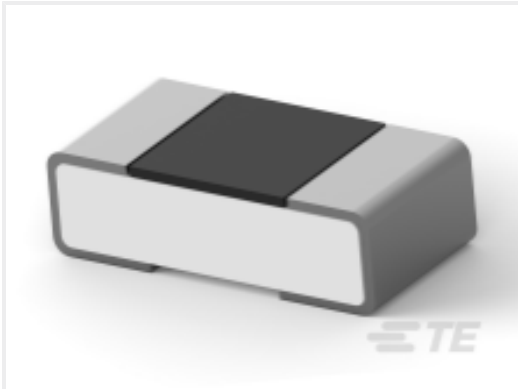
TE Part #8-2176363-2 RQ 0402 3K01 0.1% 10PPM 5K RL
