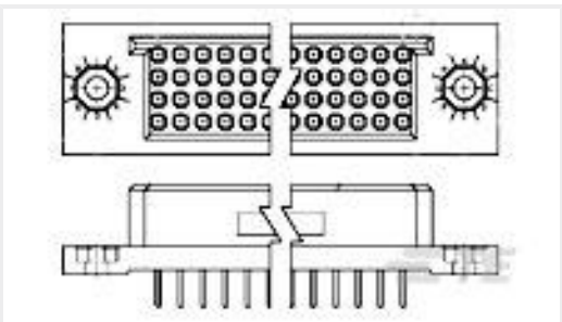
TE Part #533285-5 BOX II 4 ROW RECP ASSY 160 POS
