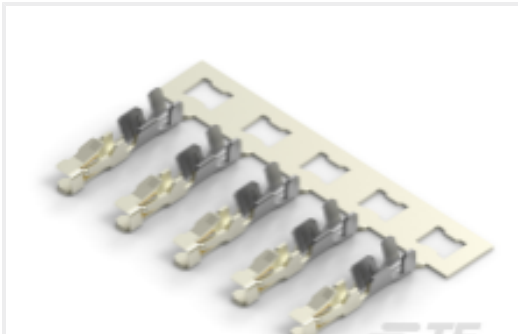
TE Part #5-2316113-5 2MM,REC,CNT,CRIMP,24-28AWG,0.76 UM,APPL
