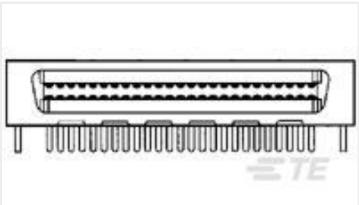
TE Part #4-5175474-2 CHAMP 050 B/B REC H W/LEG 130P
