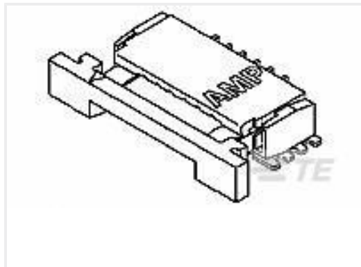
TE Part #2-84952-4 1MM FPC HORZ.BOTTOM CONT. ASSY 24P
