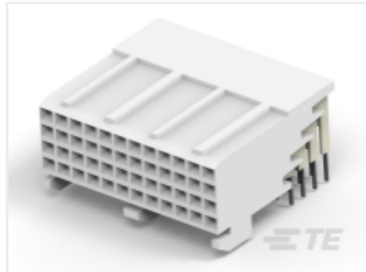
TE Part # 5536507-2 2MM FB,ASY,048,SIG,REC,SL,2.73
