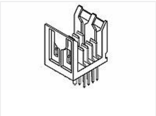
TE Part #5536600-1 2MMFB,ASY,008,PWR,HDR,SL,4.25
