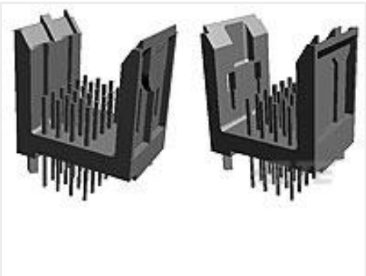
TE Part # 5536524-2 2MMFB,ASY,048,SIG,HDR,EN,5.75
