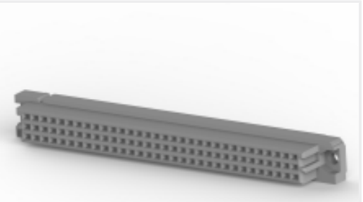
TE Part # 535059-4 064 EURO TYPE C RECEPT AP ASSY
