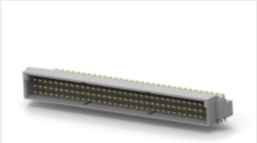
TE Part # 536366-5 096 EURO TYPE C PIN MFBLL ASSY
