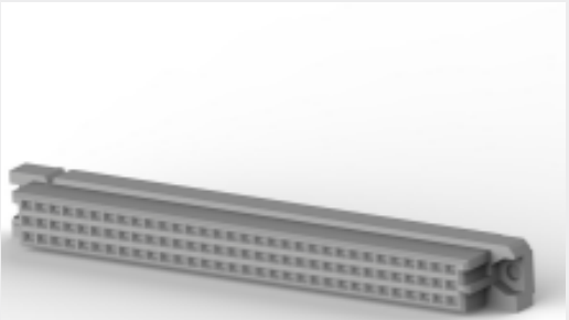
TE Part # 5650470-5 ASSY,PIN,EUROCARD,TYPE R,LEAD-
