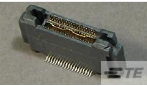
TE Part # 5767121-8 MICT,PLG,038,ASY,.025,TAPE PKG
