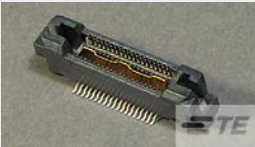
TE Part # 5767006-1 MICT,R/APLUG,38,ASSY,.025,.062
