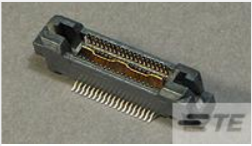
TE Part # 5767017-1 MICT,900PLUG,38,ASSY,.025,REC
