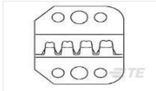
TE Part #58637-2 PRO-CRIMP DIE 20-14 UMNL
