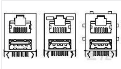
TE Part #6-1775855-3 RJ45 OVER USB W/ LED G/Y 30u" Au
