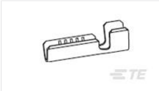
TE Part #160644-3 SPLICE 20-15 AWG .016 TPBR
