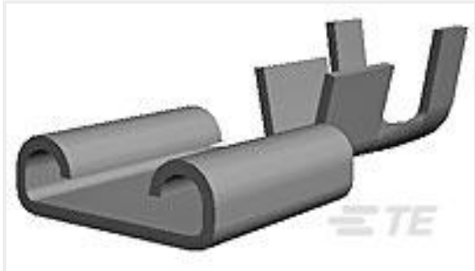
TE Part #2232723-1 PTL MFBL RECPT CONTACT, 16-19 AWG, 2X22
