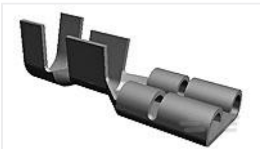
TE Part #1-2133394-1 187 FASTON HSG.,REC.,1 POS, NATRUAL
