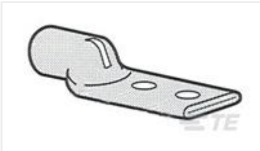
TE Part #326803 TERM, AMPOWER, 4/0, 3/8, 2 HOLE
