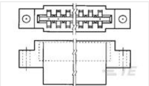
TE Part #583859-3 HOUSING CSTL 156 C/L 22 POS
