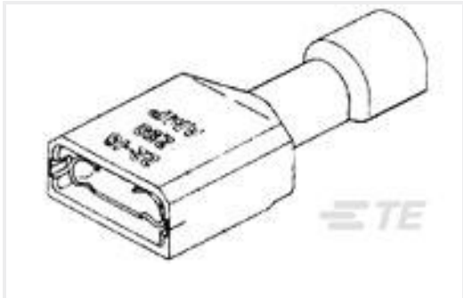
TE Part #2-520405-2 ULTRA-FAST 250 ASY REC 22-18 TPBR
