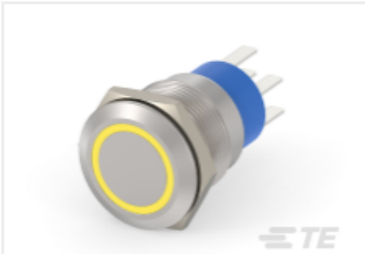
TE Part #5-2213764-1 AV19 DPM 3A FIX RING LED YELLOW 24V
