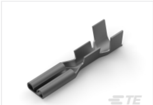
TE Part #1742785-1 110 FASTON,REC.,22-18 AWG,PTBR
