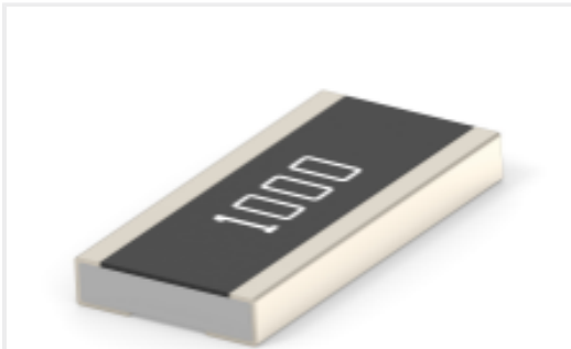
TE Part #3-2176560-8 3430 H2 1% 33R 100ppm 4k RL
