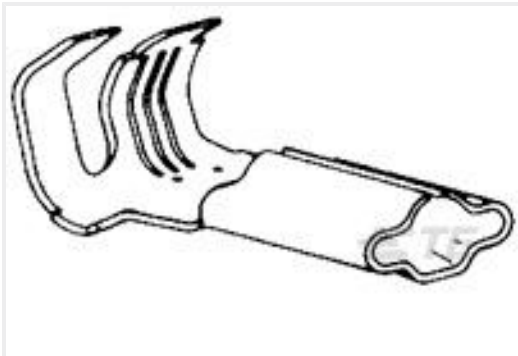
TE Part #42745-2 PIN 090 FLAG RECEPTACLE 20-14 AWG TPPHBZ
