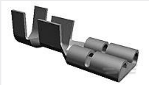
TE Part #60938-2 250 FASTON REC 18-14 AWG TPBR
