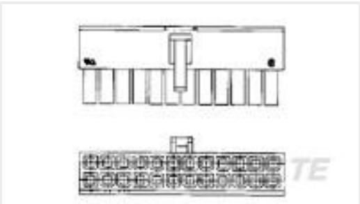
TE Part #2-1586019-4 24P RCPT VAL-U-LOK V0
