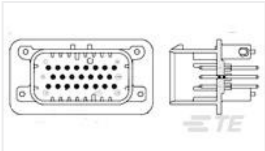
TE Part #1-776200-4 23POS,PIN DIA 1.3,HDR ASSY, 180DEG,COD 4
