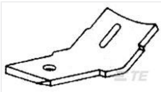
TE Part #61960-1 187 FASTON TAB NPST
