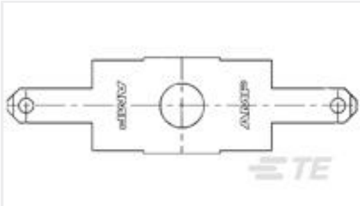
TE Part #62628-1 100 FASTON TAB TPST
