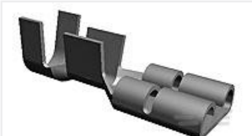
TE Part #444334-2 250 FASTON REC 22-18 AWG TPBR
