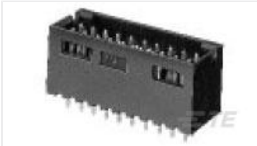
TE Part #103168-2 08 MODII HDR DRST SHRD .100CL
